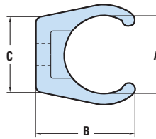
Dimensions excluding draft
