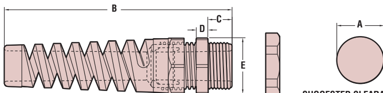
SEALING NUT WITH FLEX-PROTECTOR EXTENDER
