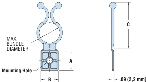
Wave Lock-Screw Mount
