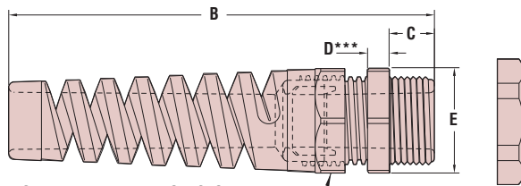
SEALING NUT WITH FLEX-PROTECTOR EXTENDER
